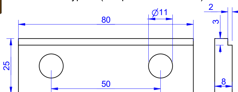
Keyplate (comparable DIN15058)
